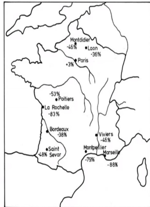
FIG. 1. The drought of spring 1788 in France. Rainfall deviation expressed as percent of the April-May 1788 rainfall compared to the mean for 1781-90. Source: Garnier (1974).
